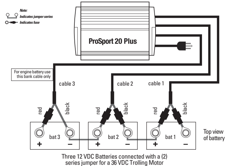
Fig. 3 ProSport 15 (OEM only) and 20 Three Bank Charger for 3 12V Batteries
