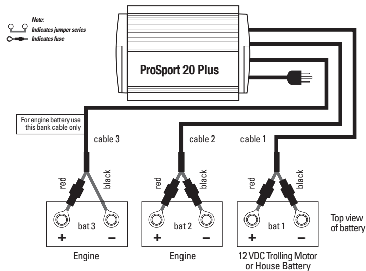
Fig. 1 ProSport 15 (OEM only) and 20 Three Bank Charger for 3 12V Batteries Dedicated 12 VDC Trolling/House Bank and 2 Engine Crank Batteries Typical Configuration
